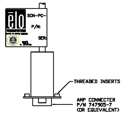
DETAIL A NOT TO SCALE ROTATED 180°
